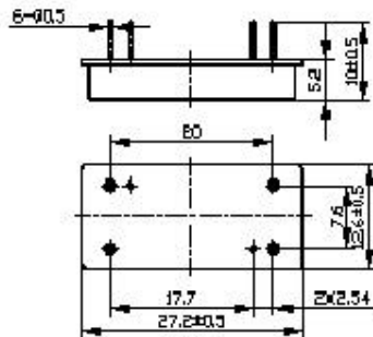
Package Outline
