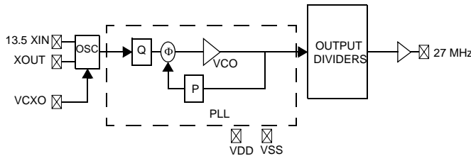
CY241V08A-01,-04 Logic Block Diagram
