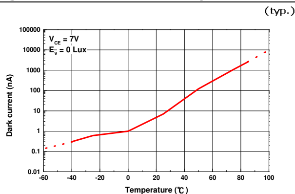
Fig.6 Dark Current vs. Temperature
