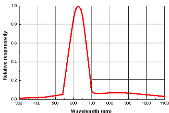
Fig.3 Spectral Response
