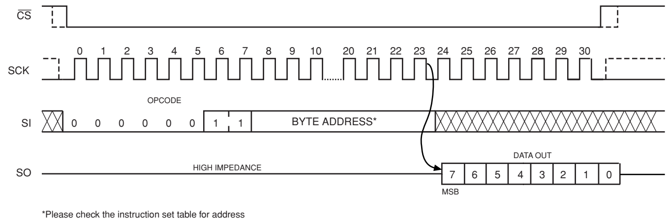
Figure 4. Read Instruction Timing
