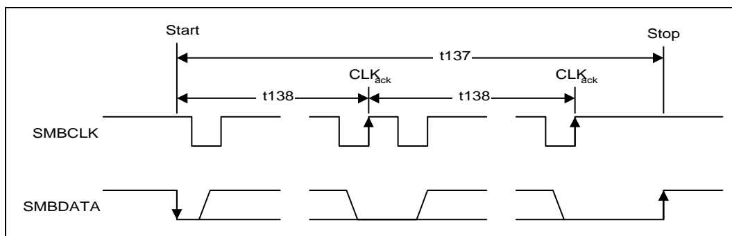
Figure 16-17. SMBus Timeout
