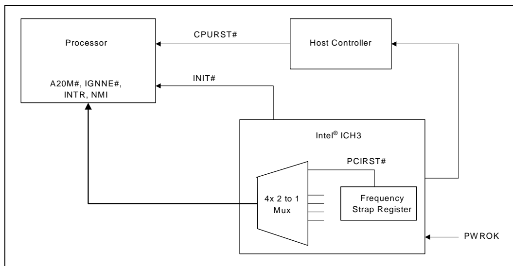
Figure 5-13. Signal Strapping
