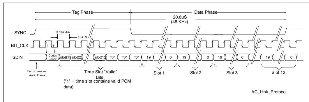
Figure 5-21. AC-Link Protocol
