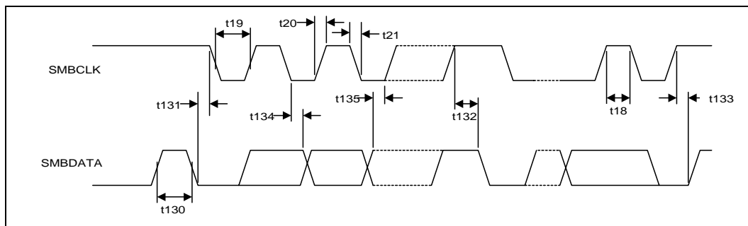
Figure 16-17. SMBus Timeout
