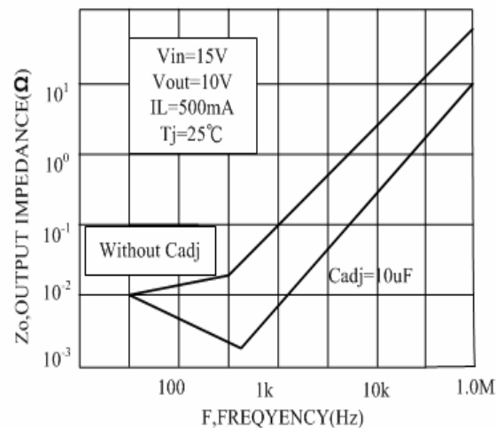
Figure10. Output Impedance
