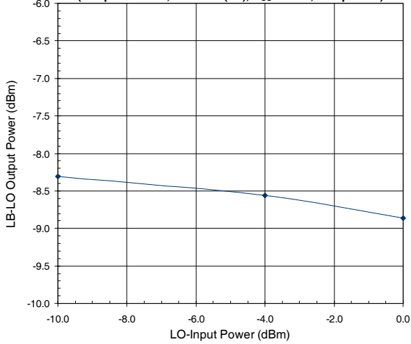
PCS Band LO Output Power versus LO-Input Power (Freq=2144MHz, V CC 2.75V, Temp 25°C)
