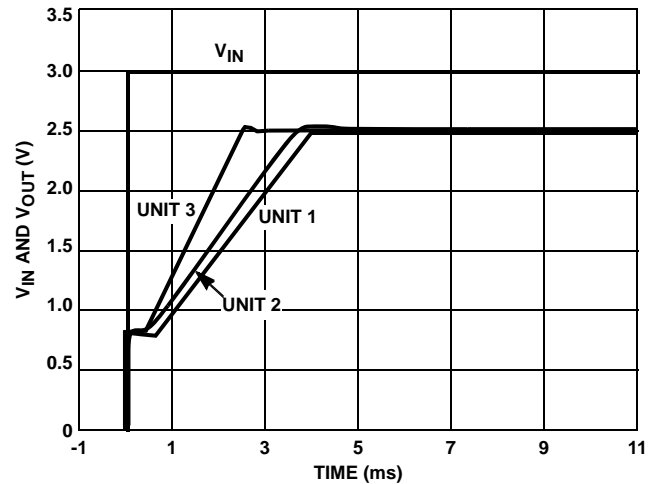
FIGURE 119. TURN-ON TIME
