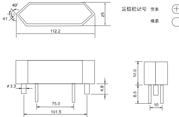
FYE-1000xZx Series
