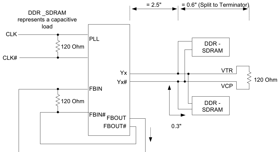
Figure 1. Clock Structure 1 [1]
