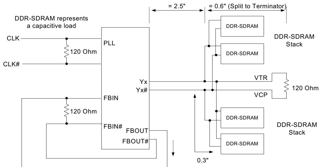
Figure 2. Clock Structure 2 [2]
