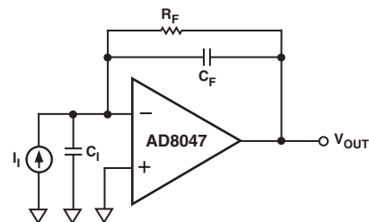
Figure 5. Transimpedance Configuration
