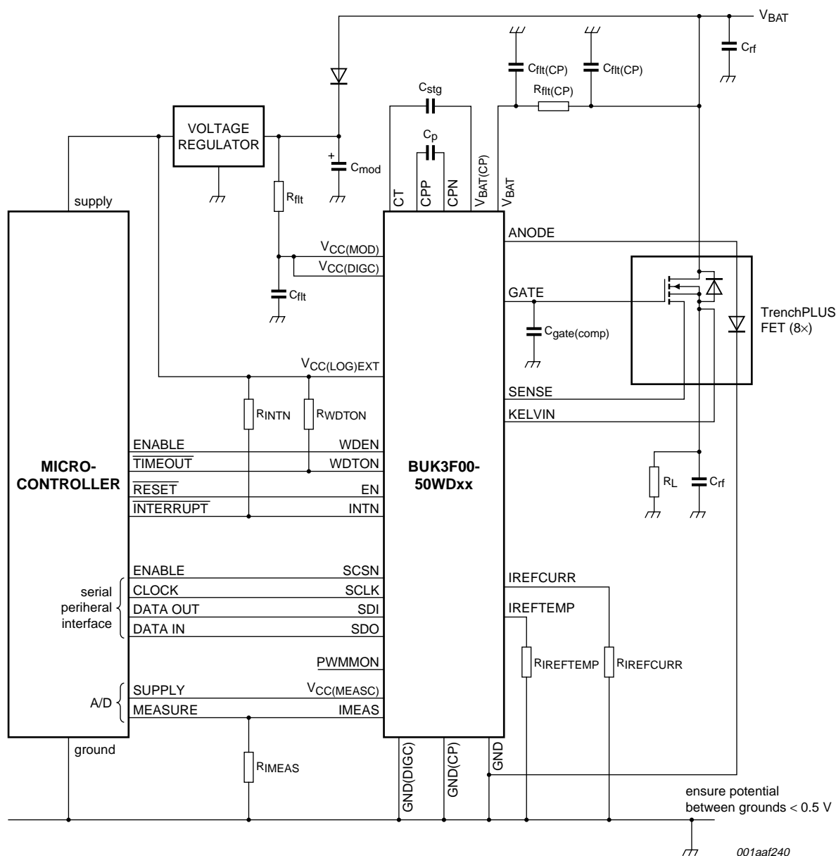
Fig 8. Application schematic
