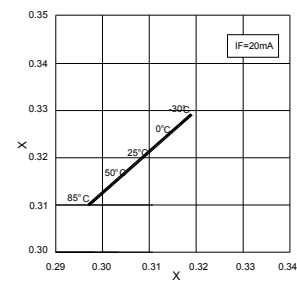
Fig.8 Ambient Temperature vs chromaticity coordinates
