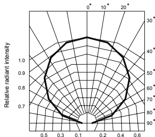
Fig.6 Radiation diagram
