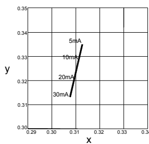
Fig.7 Forward current vs chromaticity coordinates
