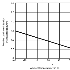
Fig.4 Relative luminous intensity vs. ambient temperature
