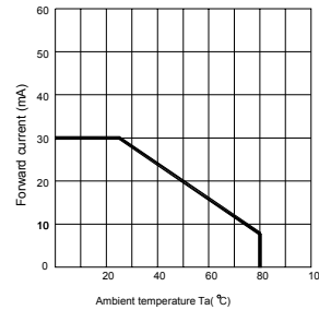
Fig.2 Forward current derating curve vs. ambient temperature
