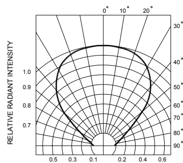
RADIATION DIAGRAM
