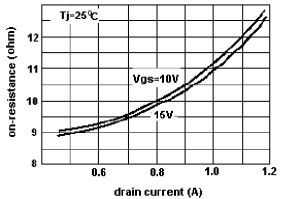
On Resistance vs Gate-Source
