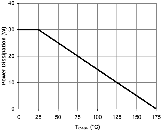
Figure 13: Power De-rating (Note B)
