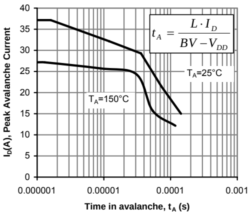
Figure 12: Single Pulse Avalanche capability
