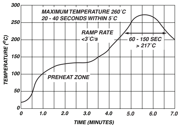
FIGURE 10. LEAD-FREE RE-FLOW SOLDER PROFILE
