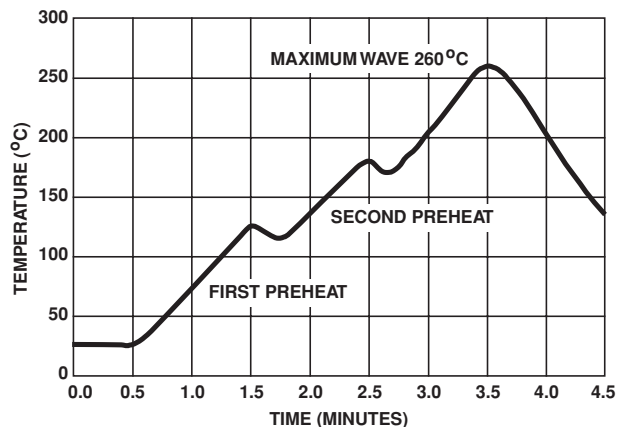
FIGURE 9. WAVE SOLDER PROFILE
