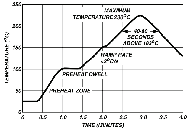
FIGURE 8. REFLOW SOLDER PROFILE
