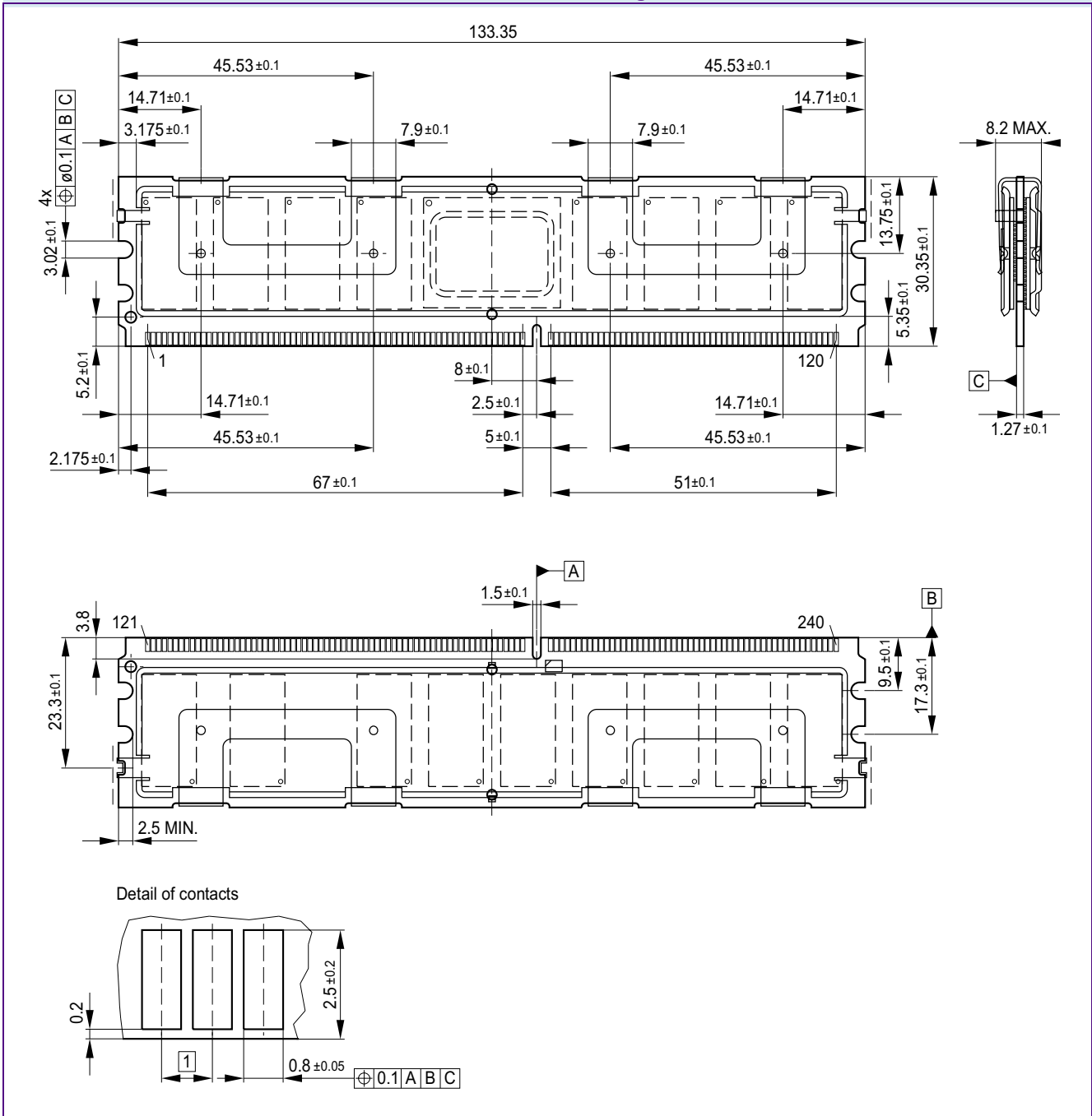
FIGURE 5 Package Outline L-DIM-240-22 with Full Heat Sink
