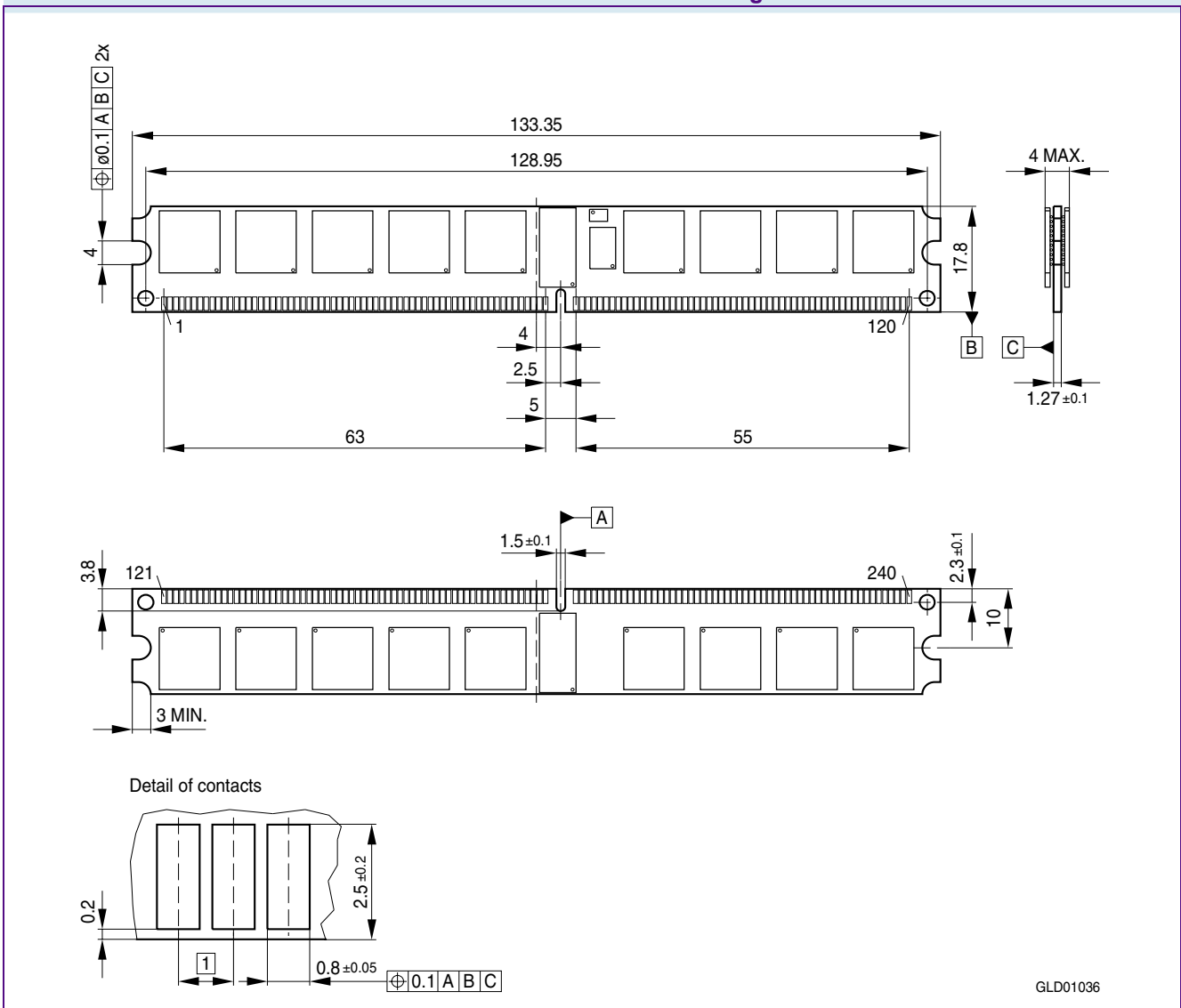
Package Outline Raw Card H - L-DIM-240-53
