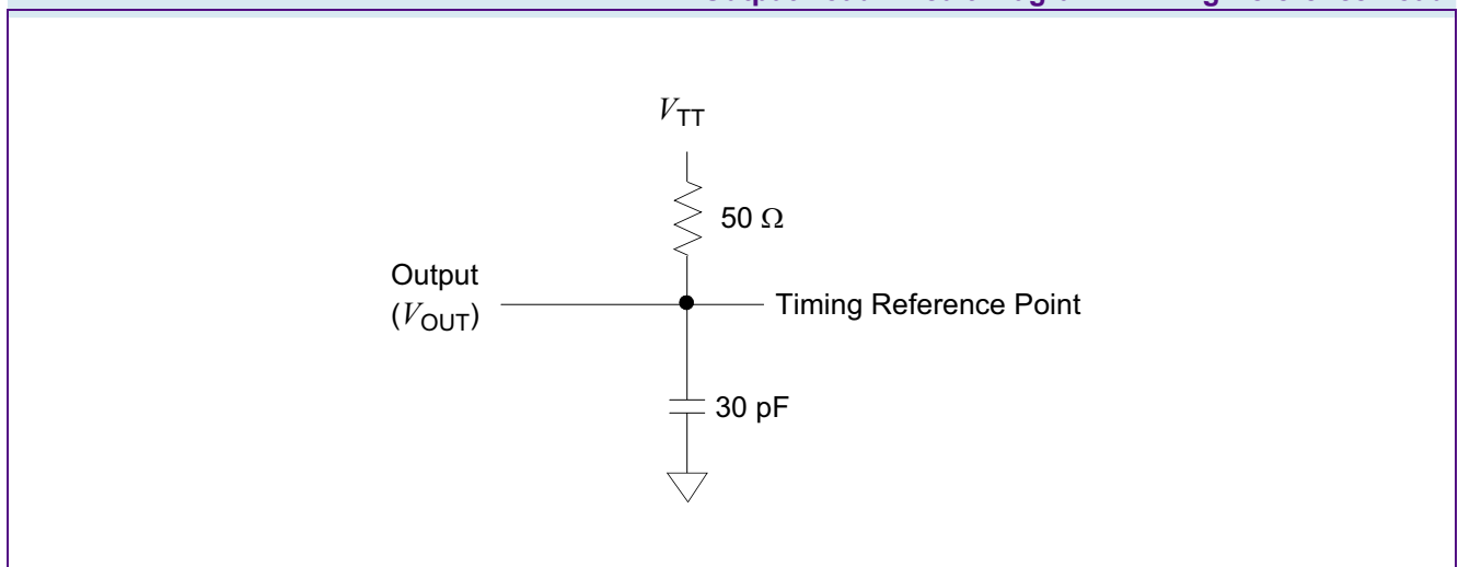
FIGURE 2 AC Output Load Circuit Diagram / Timing Reference Load
