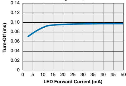
CPC1988 Typical Turn-Off vs. LED Forward Current ( I_L=0.5A )
