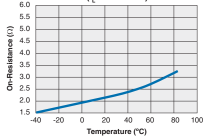
CPC1988 Typical On-Resistance vs. Temperature ( I_L=\text{max rated} )
