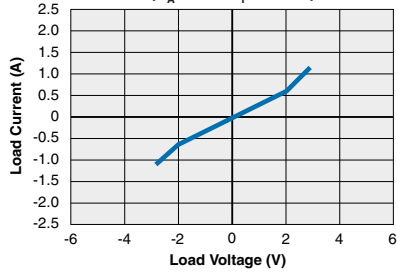
CPC1988 Typical Load Current vs. Load Voltage ( T_A=25^\circ C, I_F=10mA )
