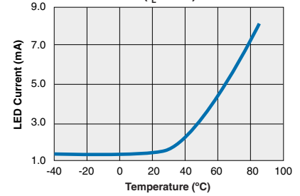
CPC1988 Typical I_F for Switch Operation vs. Temperature ( I_L=0.5A )
