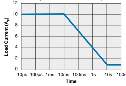
CPC1988 Energy Rating Curve (Free Air, No Heat Sink)
