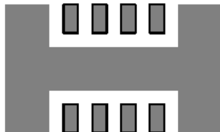
Copper Area = 50\text{mm}^2 , \theta_{JA} = 51^{\circ}\text{C}/\text{W}
