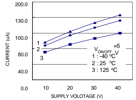
Shutdown Quiescent Current
