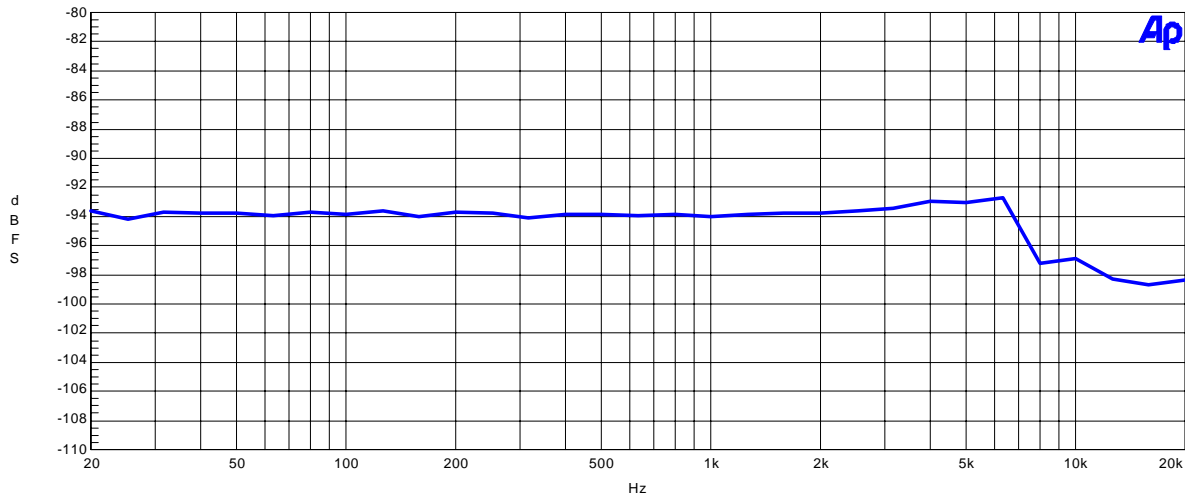
AK4584 ADC THD+N vs. Input Frequency VDD=5.0V, fs=44.1kHz, Input=-0.5dB
