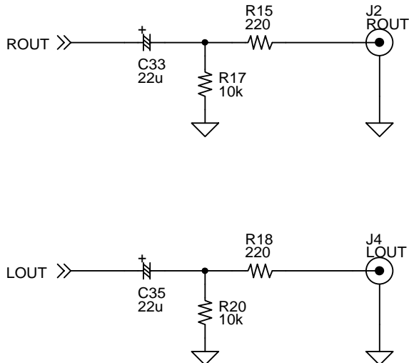
Figure 3. LOUT/ROUT Output circuits
