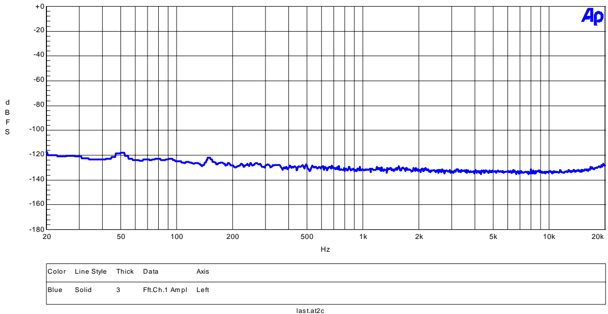
Figure 8. FFT Plot
