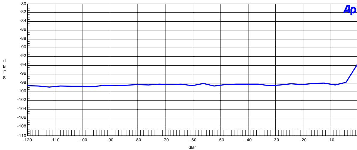
AK4584 ADC THD+N vs. Input Level VDD=5.0V, fs=44.1kHz, fin=1kHz
