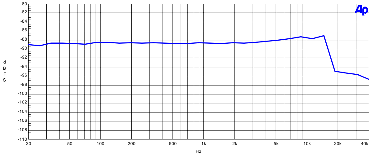
AK4584 ADC THD+N vs. Input Frequency VDD=5.0V, fs=96kHz, Input=-0.5dB
