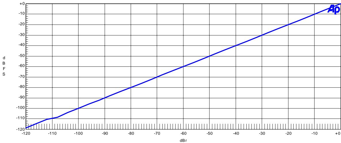
AK4584 ADC Linearity VDD=5.0V, fs=96kHz, fin=1kHz
