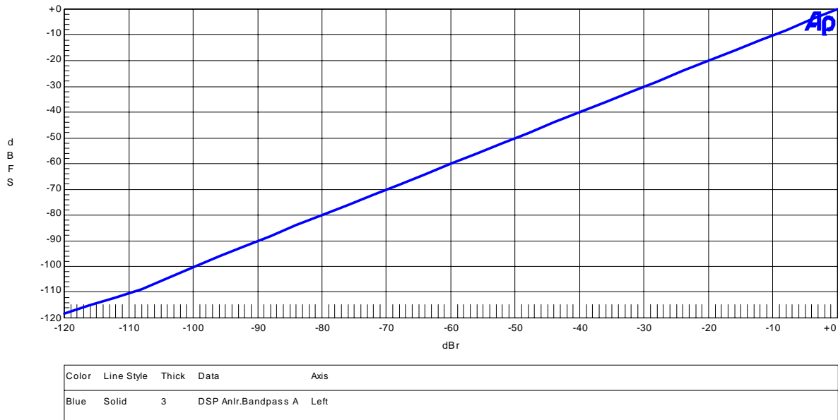
Figure 3. Linearity
