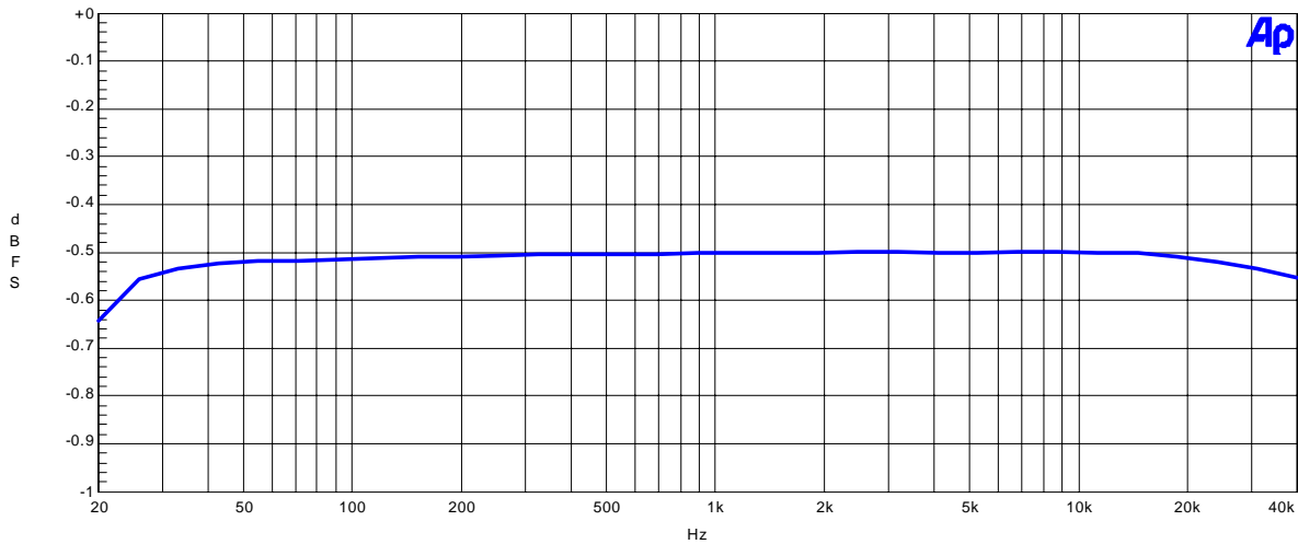
AK4584 ADC Frequency Response VDD=5.0V, fs=96kHz, Input=-0.5dBr
