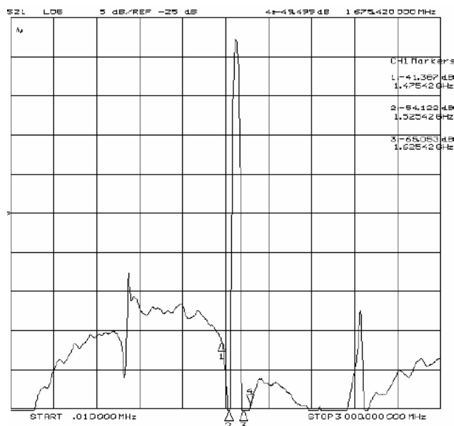
Frequency Response
