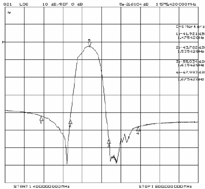
Frequency Response
