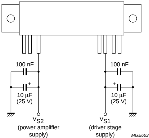
Fig.5 Recommended decoupling arrangement.
