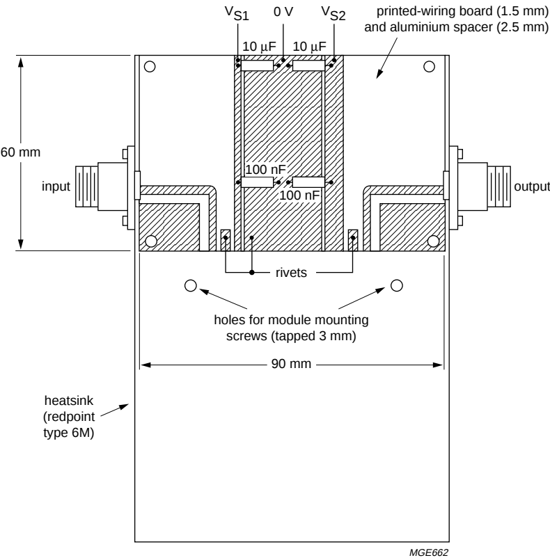
Fig.4 Test jig for VHF modules.
