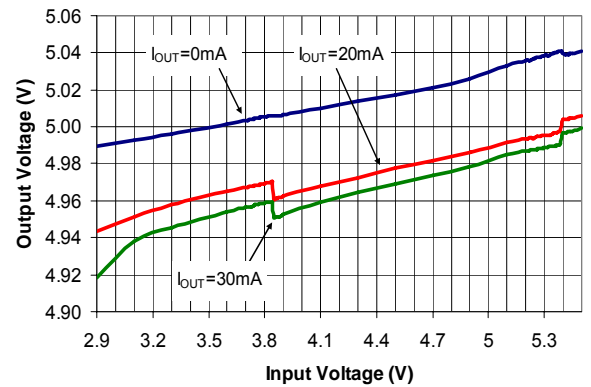
Figure 14. Line Regulation
