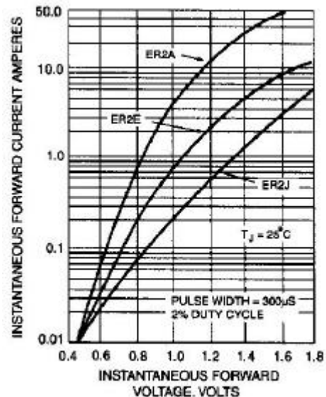
Fig. 4-TYPICAL FORWARD CHARACTERISTICS
