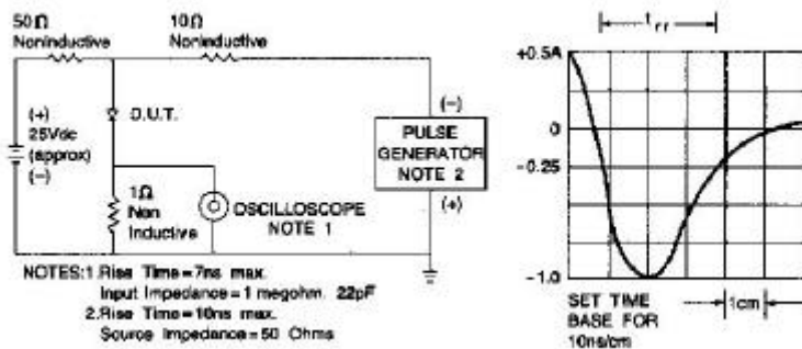
Fig. 1-REVERSE RECOVERY TIME CHARACTERISTIC AND TEST DIAGRAM
