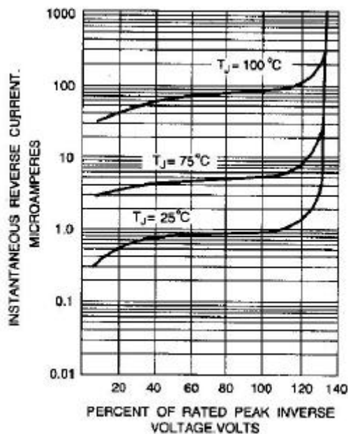
Fig. 3-TYPICAL REVERSE CHARACTERISTICS
