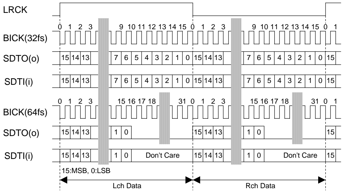
Figure 19. Mode 2 Timing
