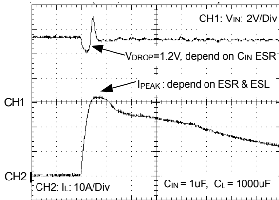
Time (25us/Div)
