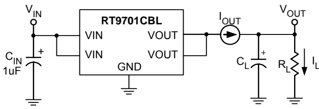
Test Circuit 1
