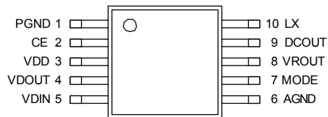
MSOP-10 (TOP VIEW)
