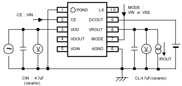
Circuit 12 Ripple Rejection Rate
