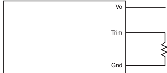
Trim Up Test Circuit
