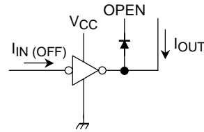
4. I_{IN(OFF)}
