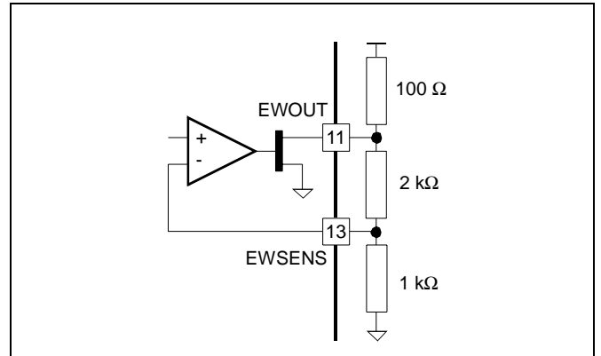
Figure 7: E/W Output
