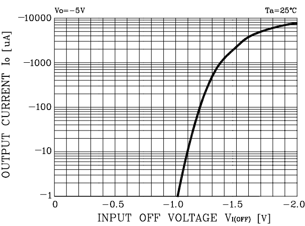
Fig. 2 I_O - V_{I(OFF)}
