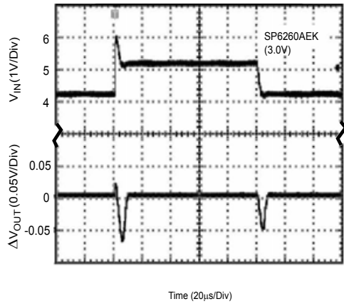
SP6260EEK (3.0V) Line Transient (Conditions: I_{OUT}=30\text{mA} , C_{IN}=1\mu\text{F} , C_{OUT}=1\mu\text{F} )
