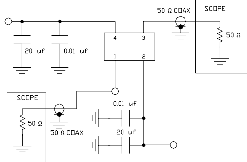
TEST CIRCUIT
