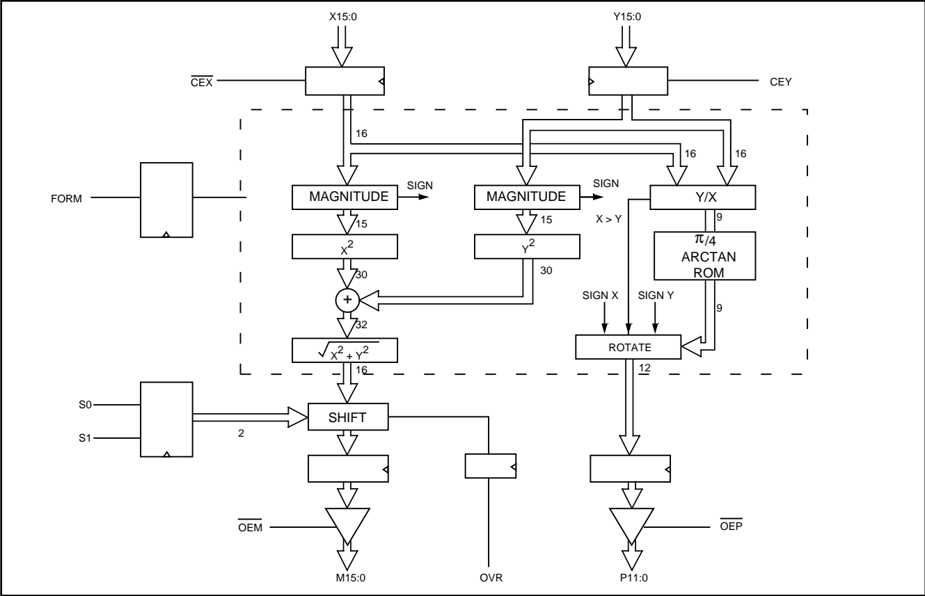
Fig.2 Block diagram
