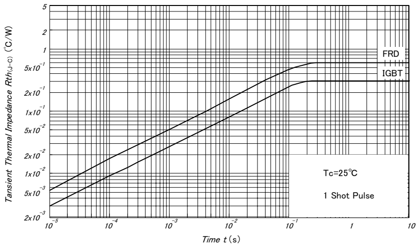
fig11-Tansient Thermal Impedance
