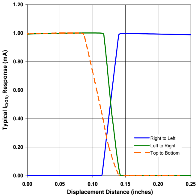
OPB816Z - Flag in Middle of Slot
