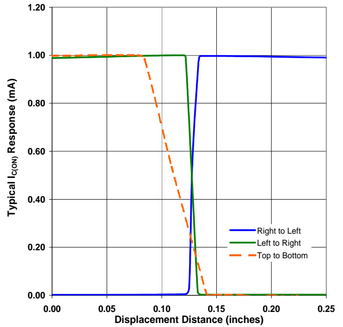
OPB816Z - Flag Next to Sensor
