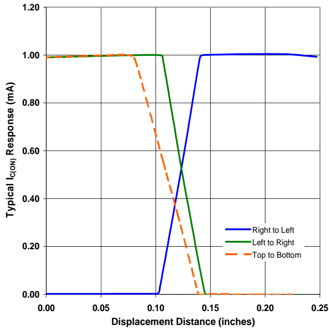
OPB816Z - Flag Next to Emitter
