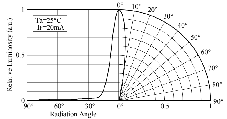
■ Directivity (NSPG500(S))
