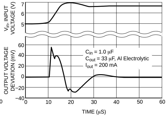
Figure 11. Line Transient
