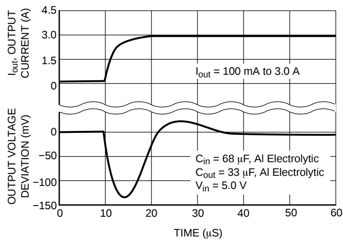
Figure 12. Load Transient
