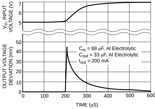
Figure 10. Line Transient
