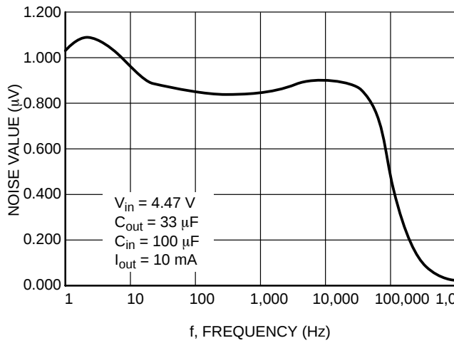
Figure 8. Noise Characterization
