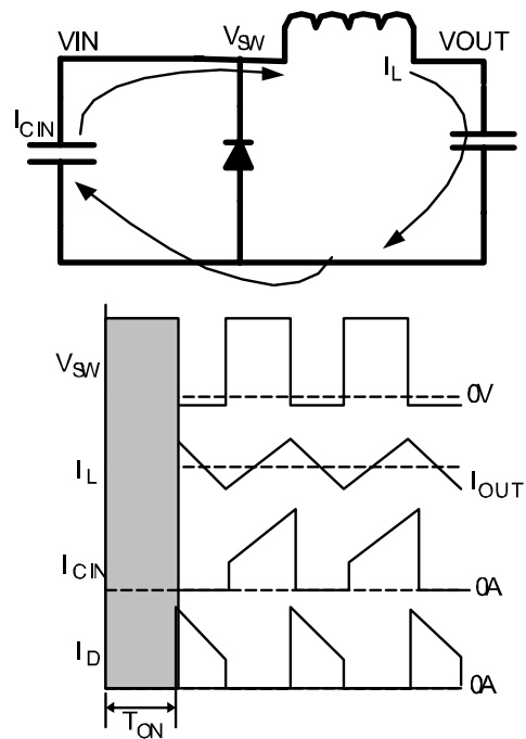
Figure 3. On-Time
