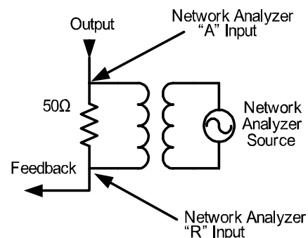
Figure 7. Transformer Injection
