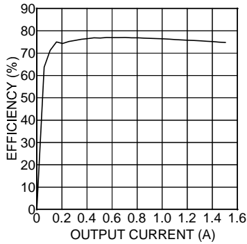
5V IN to 1.8V O Efficiency
