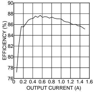
3.3V IN to 1V O Efficiency
