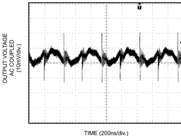
Output Ripple
