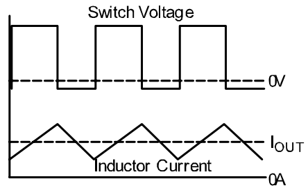
Figure 2. Continuous Operation
