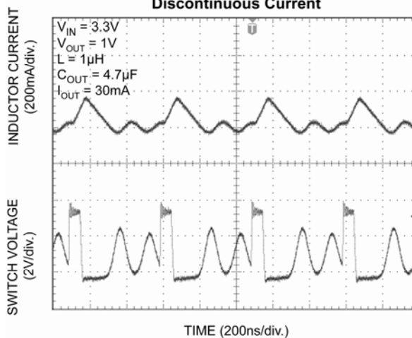
Discontinuous Current
