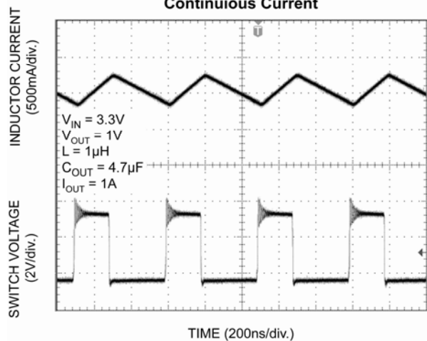
Continuous Current
