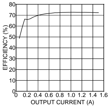
5V IN to 1V O Efficiency
