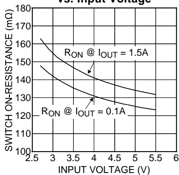
Switch On-Resistance vs. Input Voltage
