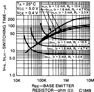
Fig. 12. Switching Time vs. R_{BE}
