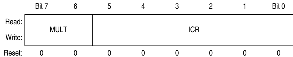
Figure 13-6 IIC Frequency Divider Register (IICF)
