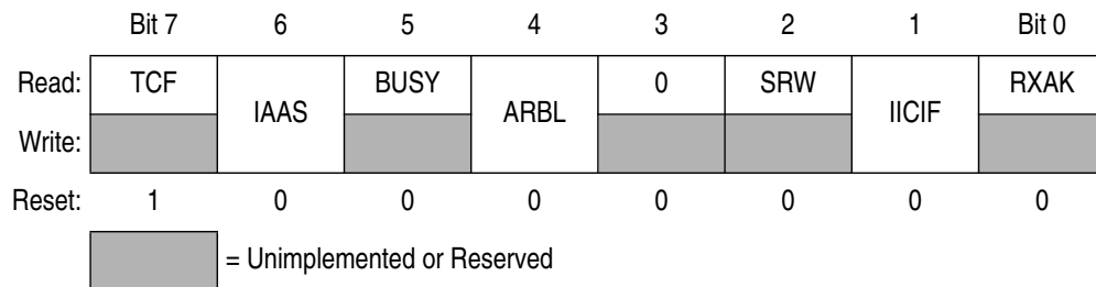
Figure 13-8 IIC Status Register (IICS)
