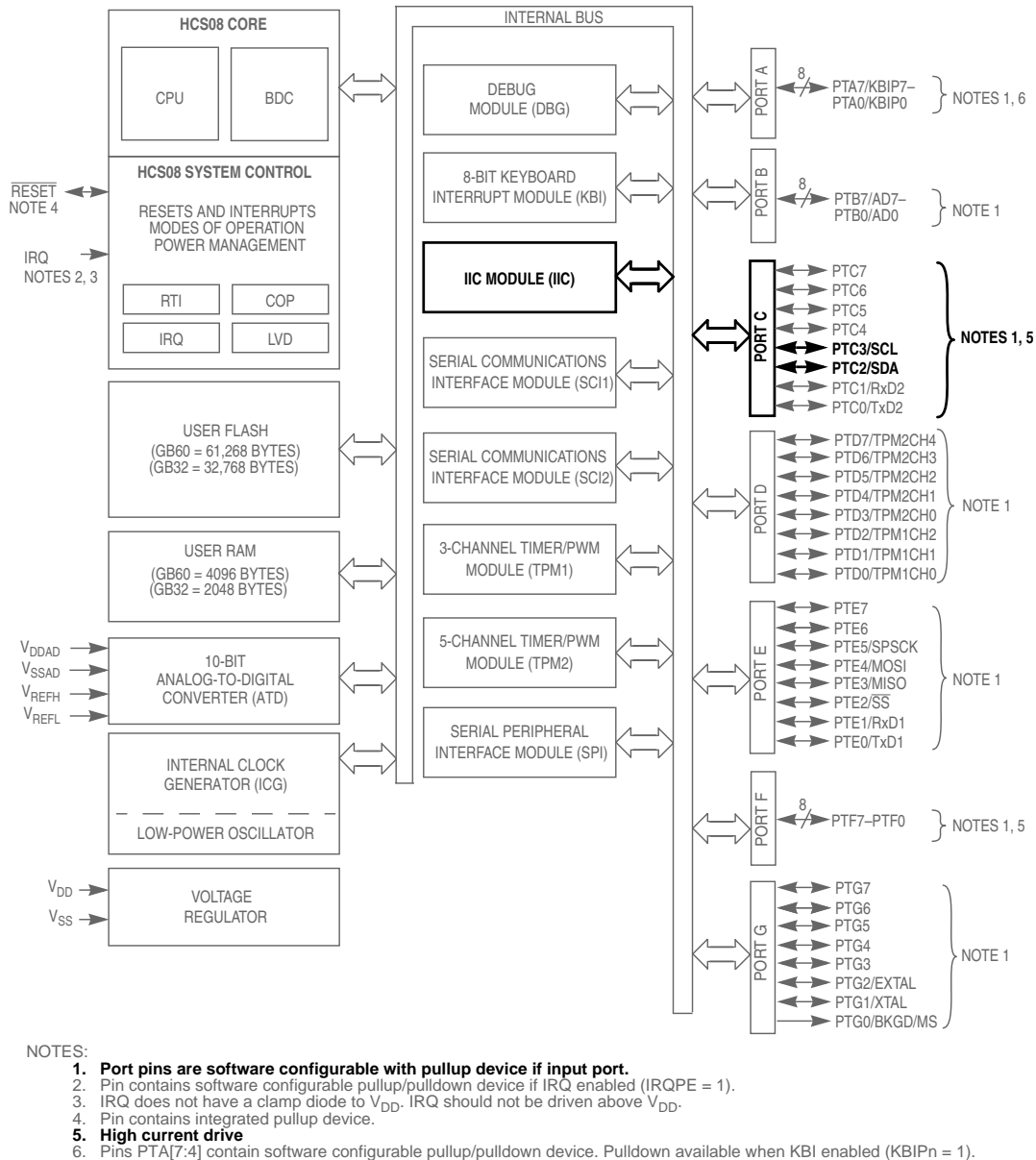
Figure 13-1 Block Diagram Highlighting the IIC Module
