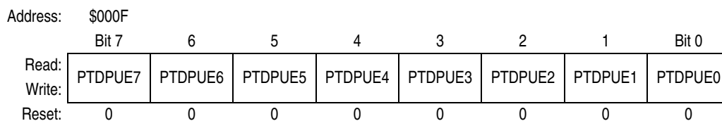
Figure 12-16. Port D Input Pullup Enable Register (PTDPUEx)
