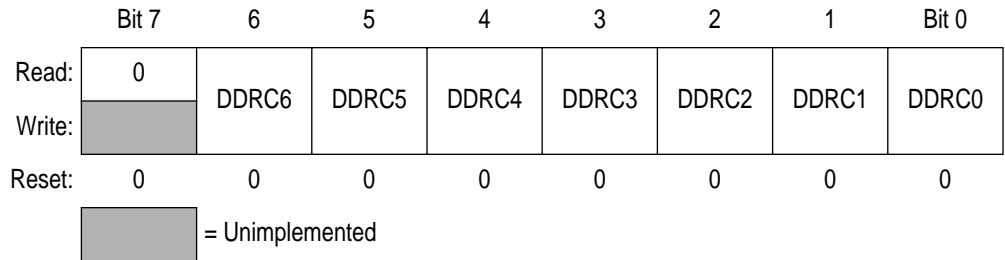
Figure 15-10. Data Direction Register C (DDRC)
