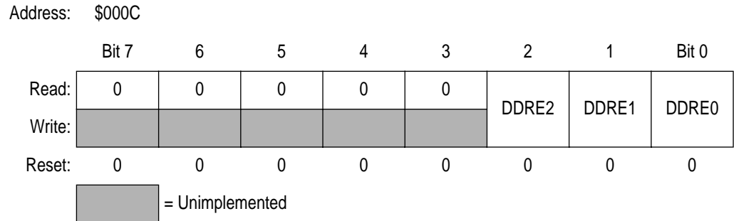
Figure 15-17. Data Direction Register E (DDRE)
