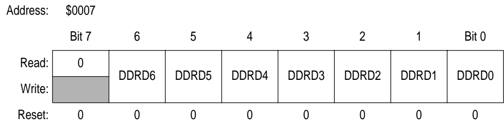
Figure 15-13. Data Direction Register D (DDRD)
