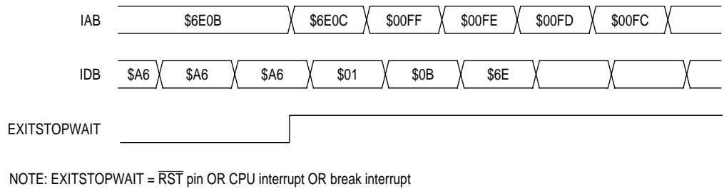
Figure 7-14. Wait Recovery from Interrupt or Break
