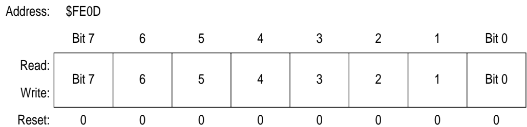
Figure 18-4. Break Address Register Low (BRKL)
