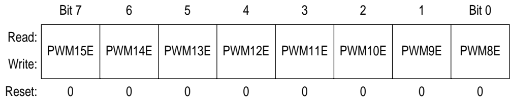
Figure 15-4. PWM Control Register 1 (PWMCR1)
