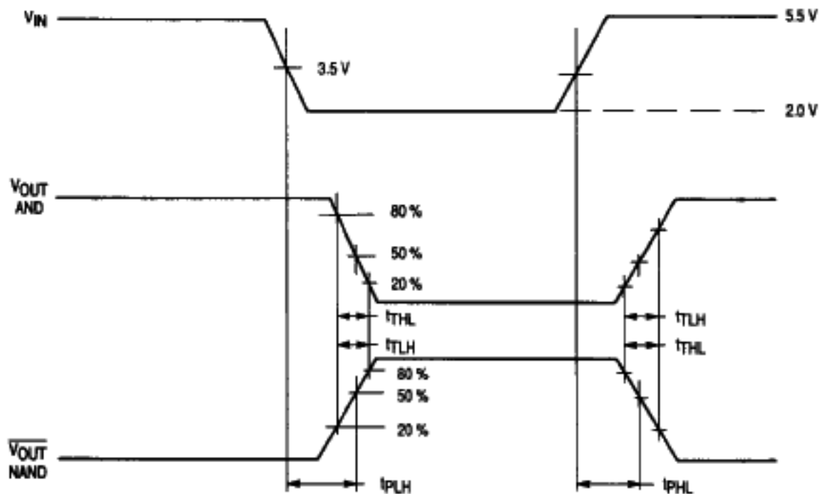
Figure 1. Switching Test Circuit and Waveforms
