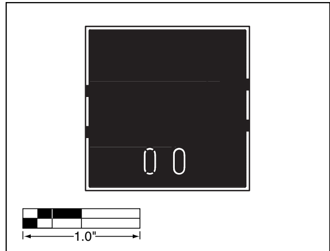
Figure 5. MAX2644 EV Kit PC Board Layout—Ground Plane Layers 2 and 3
