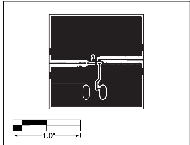
Figure 3. MAX2644 EV Kit PC Board Layout—Component Side
