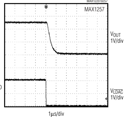
NEGATIVE FULL-SCALE SETTLING TIME R_{LOAD} = 10k\Omega , C_{LOAD} = 100pF
