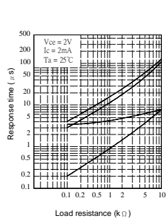
Response time Vs. Load resistance
