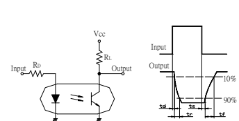
Test circuit for response time
